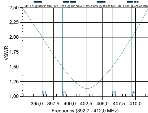
TYPICAL VSWR A-300MU
